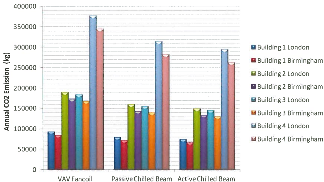
Fig 8. HVAC Plant Annual CO2 Emission
